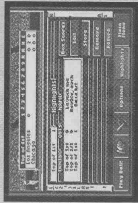
Fig. 20 Highlights Screen
